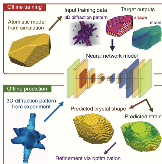
Figure 2-1 AI workflow for Bragg CDI data inversion.
