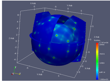
Figure 2-8 Visualization of a dataset from a pixel from a Silicon analyzer crystal processed with RSM3D. This data shows a combination of diffraction (bright spots) and thermal diffuse scattering (broad lines connecting diffraction spots). This data was taken on the High Energy Resolution Inelastic X-Ray Spectrometer (HERIX) at APS Sector 30.
