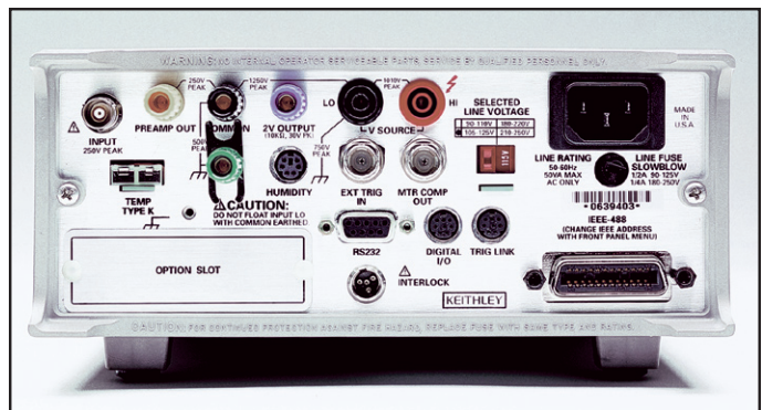
Model 6517A rear panel
