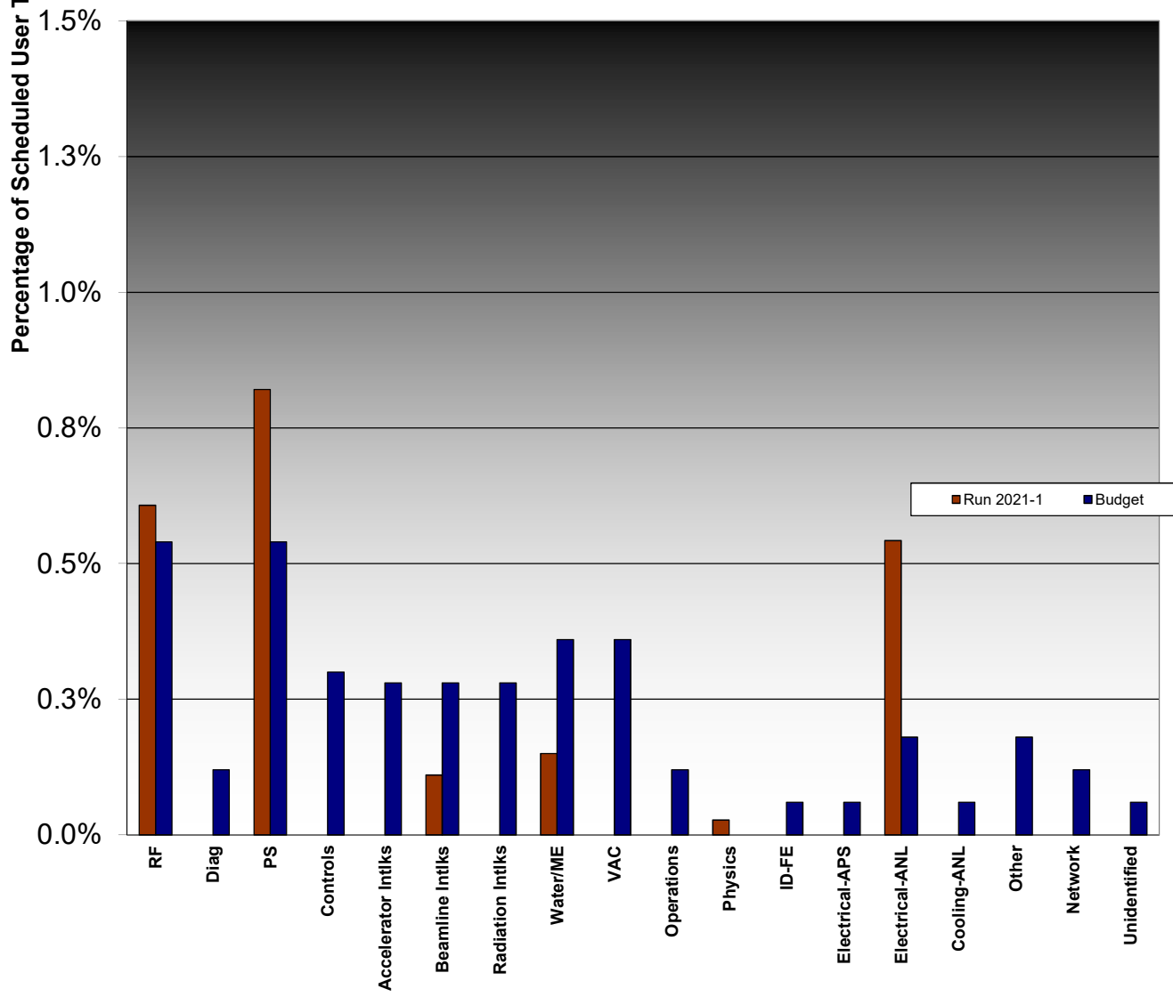
Run 2021-1 Downtime by System January 26, 2021-April 22, 2021 Scheduled User Time = 1767 hours User downtime = 39.90 hours
