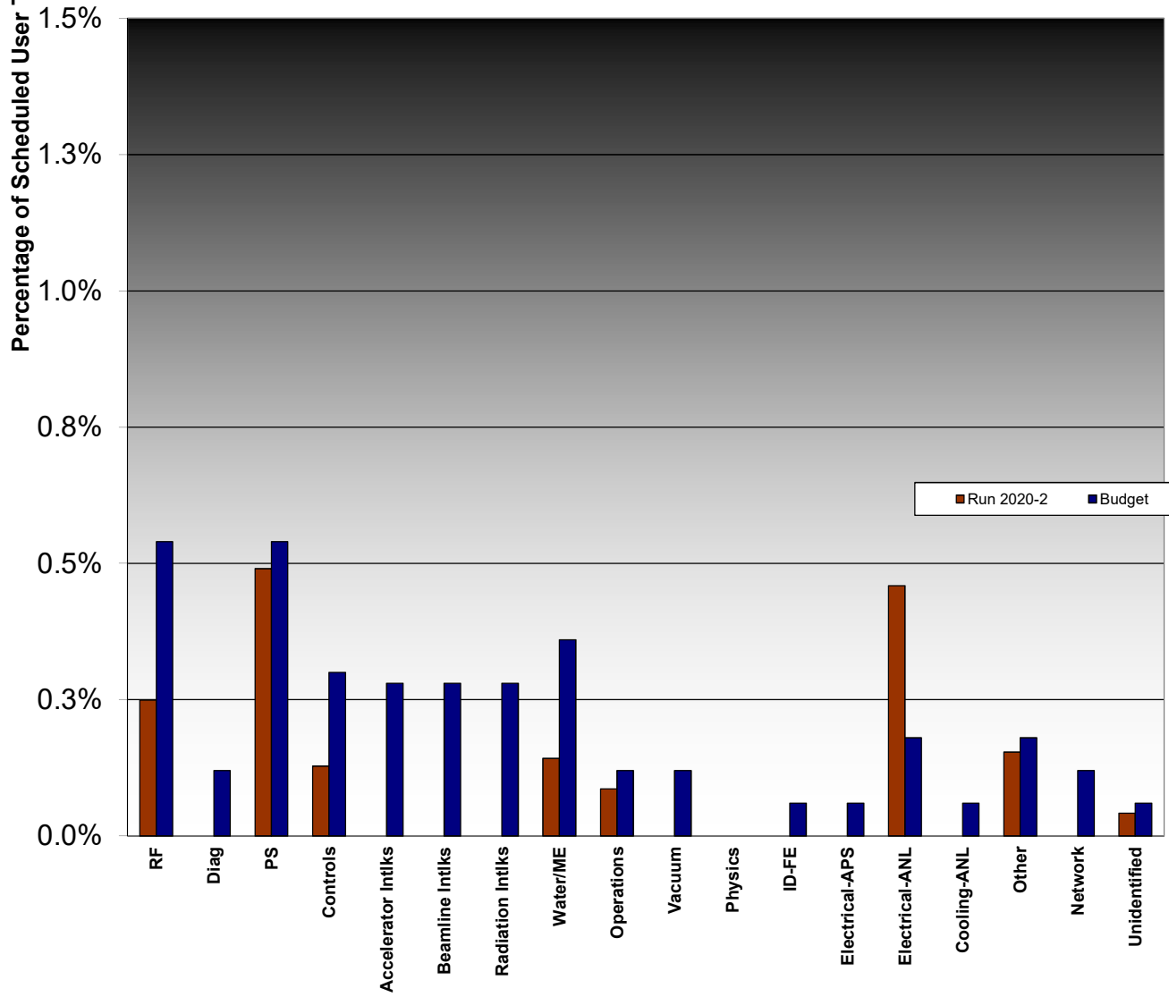
Run 2020-2 Downtime by System June 16 - September 28, 2020 Scheduled User Time = 1431 hours User downtime= 27.23 hours
