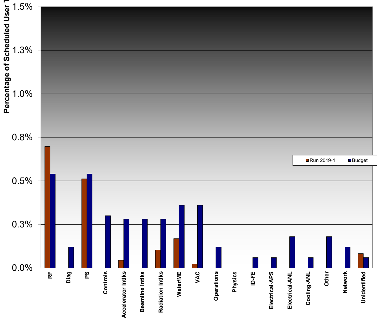
Run 2019-1 Downtime by System January 29 - April 22, 2019 Scheduled User Time = 1719 hours User downtime = 28.03 hours
