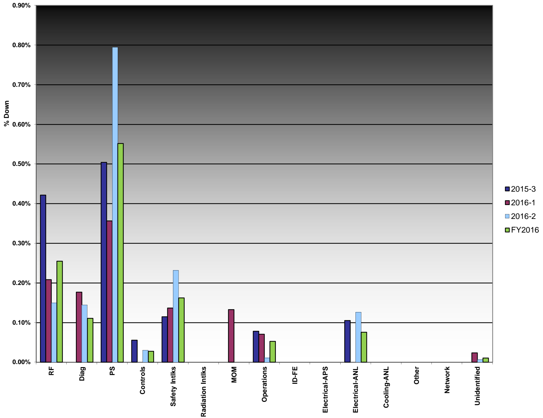
FY 2016 Downtime by System Data through Run 2016-2
